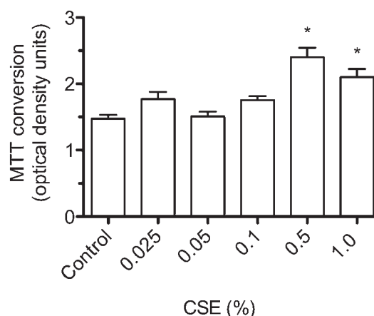
Figure 1 Conversion of MTT (3-(4,-dimethylthiazol-2-yl)-2, 5-diphenyl-tetrazolium) by A459 cells stimulated with cigarette smoke extract (CSE) for 4 h. Optical density (OD) of the formazin product is detected by spectroscopy at 550 nm. CSE does not attenuate in the ability of cells to convert MTT, indicating an absence of cytotoxicity. CSE increased conversion at 0.5 and 1% (*p<0.05 vs medium control).
