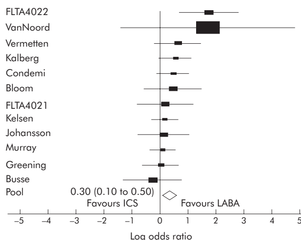
Figure 3 Odds ratio for number of subjects with one or more moderate or severe exacerbation. Forest plot of fixed effects. ICS, inhaled corticosteroids; LABA, long acting \beta agonist.
