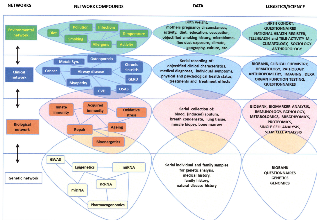
Figure 1 Network medicine in airway disease (modified with permission from Agusti and Vestbo 35 ). Diagram illustrating the different levels of complexity of airway disease. At each level, only some of the potential components are shown to illustrate the concept (the diagram is not intended to be comprehensive). Likewise, links between the different elements of the network are drawn for illustrative purposes only and do not necessarily reflect evidence-based relationships. The middle and right-hand column respectively show the data required and the logistics and scientific knowledge needed to perform a study on a new taxonomy of airway disease. For further explanations, see text. CVD, cardiovascular disease; GERD, gastroesophageal reflux disease; GWAS, genome-wide association studies; M, monitoring; miDNA, mitochondrial DNA; miRNA, microRNA; ncRNA, noncoding RNA; OSAS, obstructive sleep apnoea syndrome.
